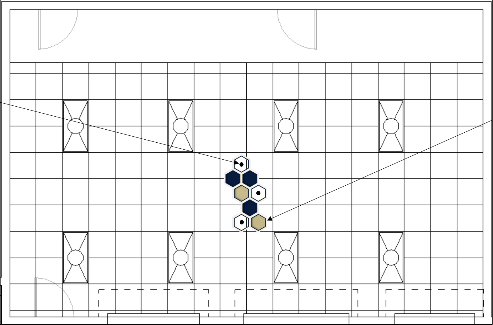
SERVING ROOM REFLECTED CEILING PLAN
